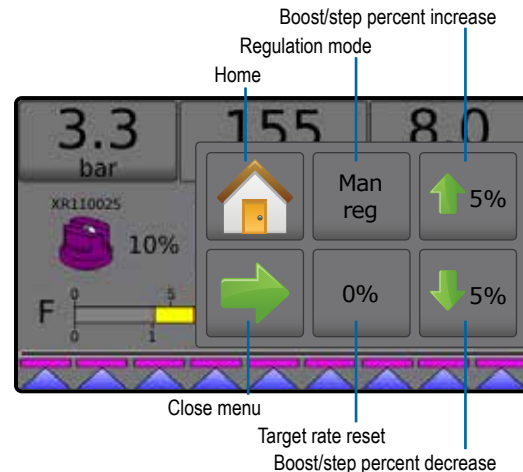
Figure 5: Options tab – Manual mode
