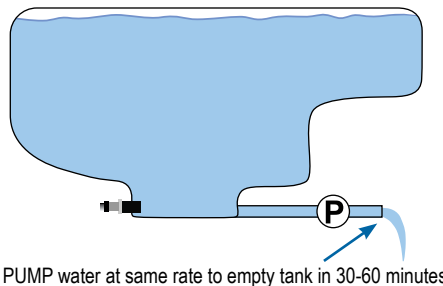
Figure 38: Tank shape calibration
