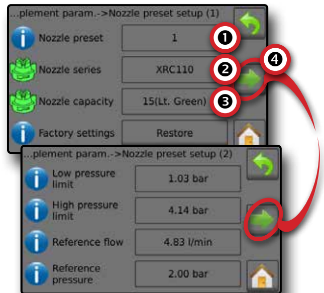
Figure 52: Establish nozzle presets
