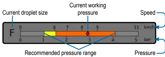
Figure 56: Pressure gauge example
