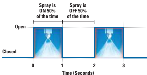
Precision Spray Control (PSC) turns nozzles on and off quickly to control flow rate. With traditional nozzles, flow rate adjustments require a change in liquid pressure, which also changes the nozzle's spray angle/coverage and droplet size. With PSC, pressure remains constant, enabling flow rate changes without affecting spray performance. This reduces the use of costly coatings by applying the proper volume directly on the boards.
